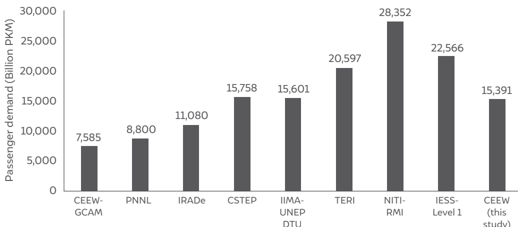
Figure 9 A comparison of projected passenger travel demand and energy demand in 2030 by various models with our estimate
