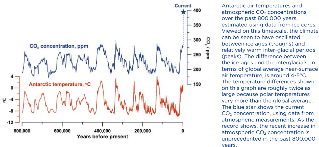
Figure 2: The last 800,000 years. Changes in Antarctic air temperatures and atmospheric CO 2 concentrations 2
