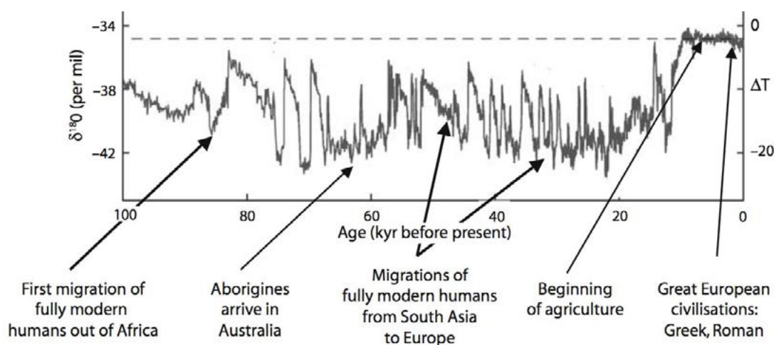
Figure 3: The last 100,000 years Temperature change, as measured in Greenland 3
