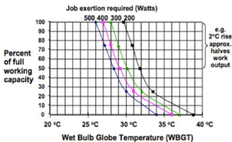
Figure 1: The relationship between heat and work - a function of ideal human physiology and a pointer to fundamental temperature thresholds. 9
