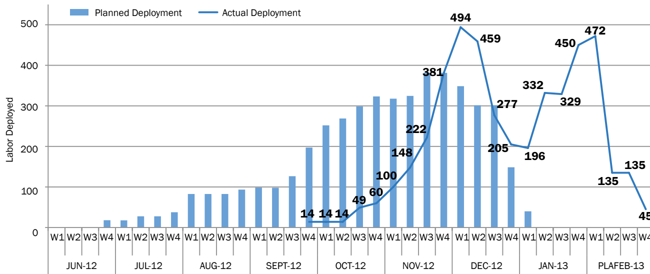
Figure 1: Solar PV Project Construction Activity, Planned Vs. Actual
