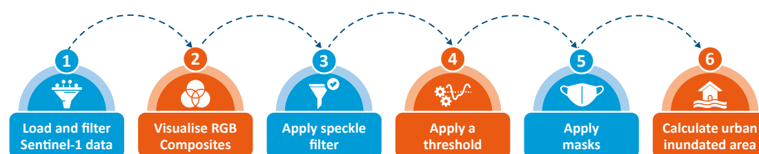
Figure 6: Flood inundation mapping carried out through a series of systematic steps
