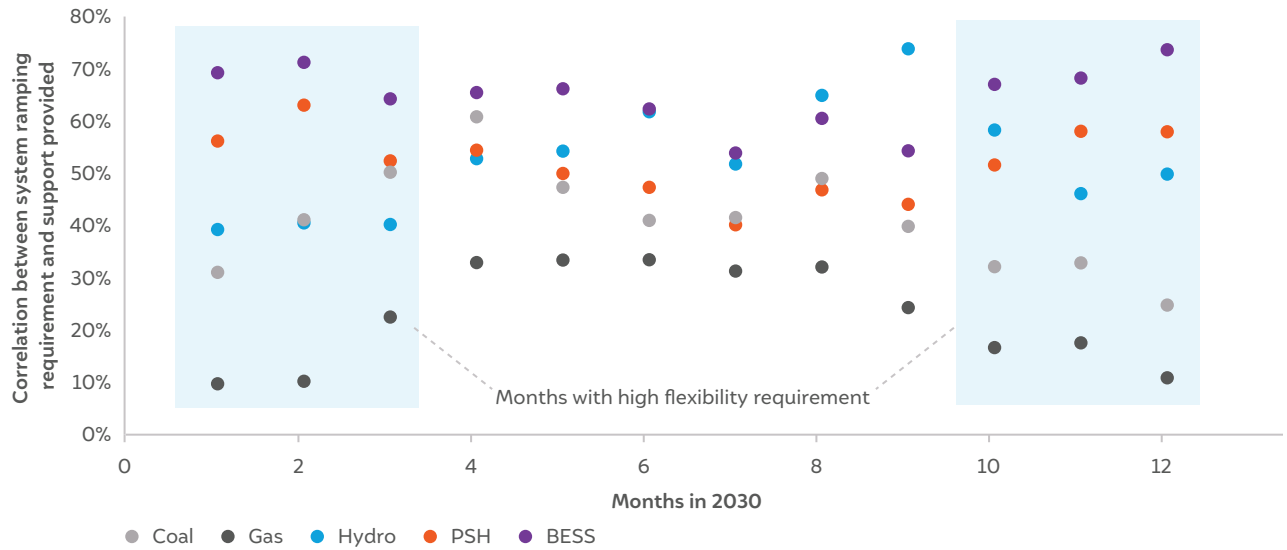
Figure 11 BESS supports high system ramping requirements
