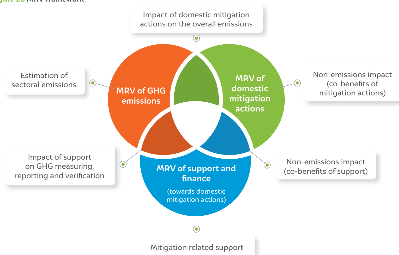
Figure 28 MRV framework
